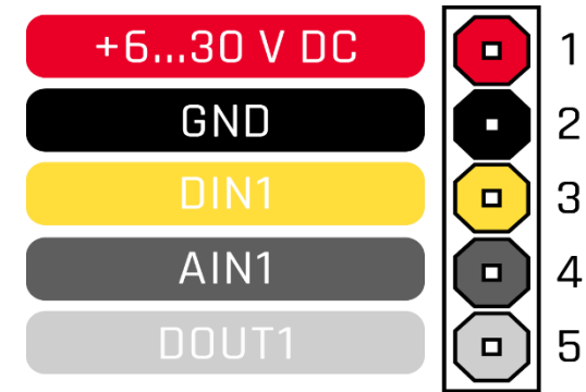
Figure 2 FMB910 pinout
