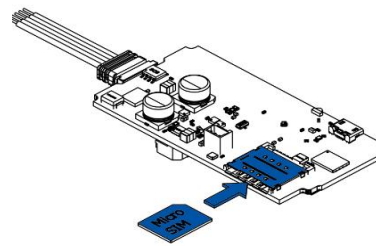
3 Figure 6 Micro SIM card insert
