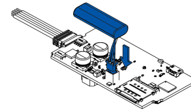
2 Figure 5 Wiring harness connection
