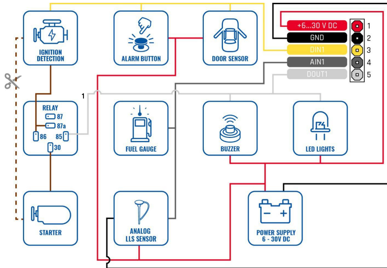
Figure 3 FMB910 Wiring scheme
