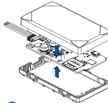
5 Figure 8 Attaching cover back
